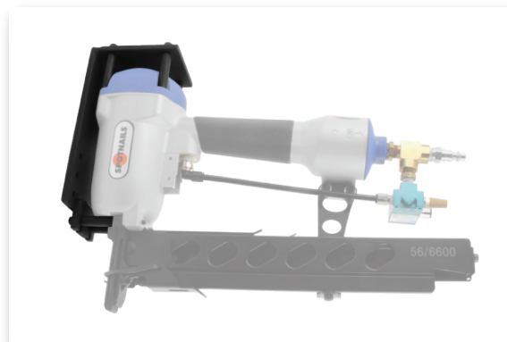
Angle Mounting System for W1 Body Style Tools (Left and Right)
