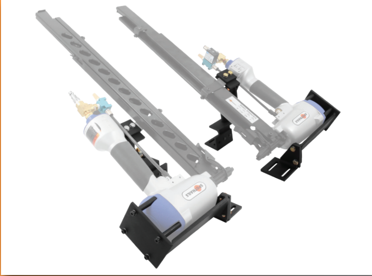
Angle Mounting System for X1 Body Style Tools (Left and Right)
